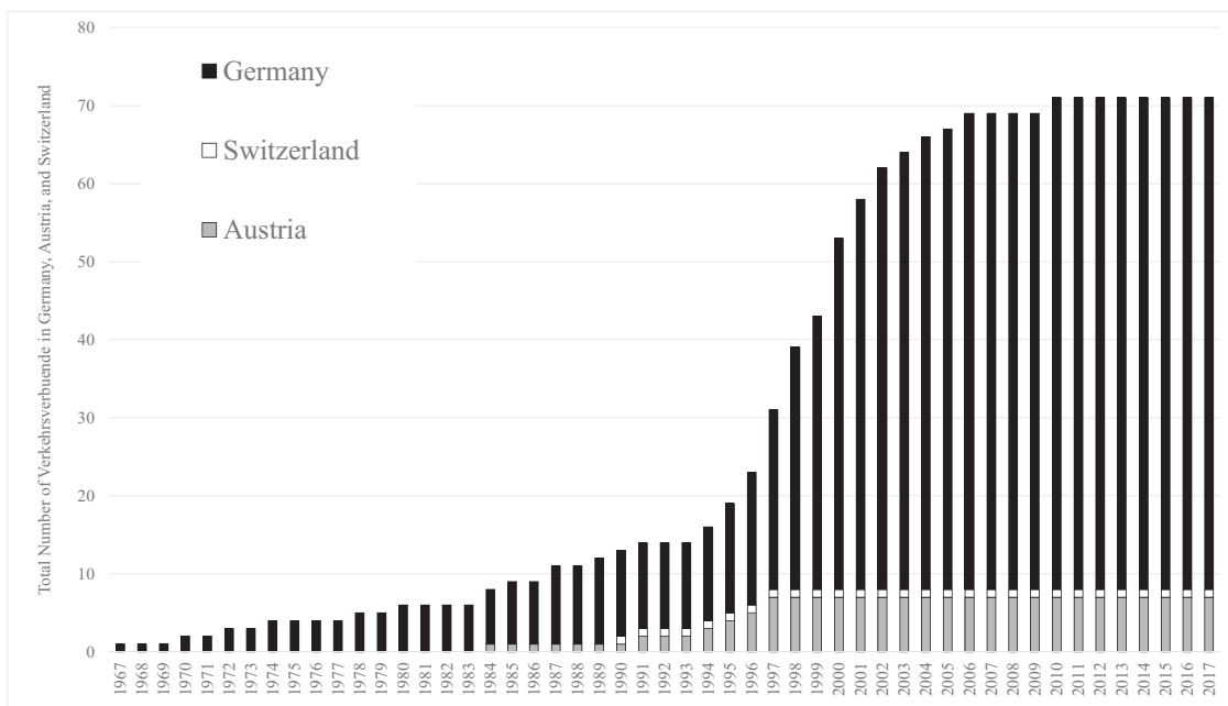
Figure 1. Expansion of Verkehrsverbünde in Germany, Austria, and Switzerland, 1967–2017. Sources: Based on information in Dümmmler, 2015; Koch and Newmark, 2017; VDV, 2009. Note: The graph only includes VVs currently in operation, thus excluding VVs that no longer exist because of their amalgamation into larger VVs.
